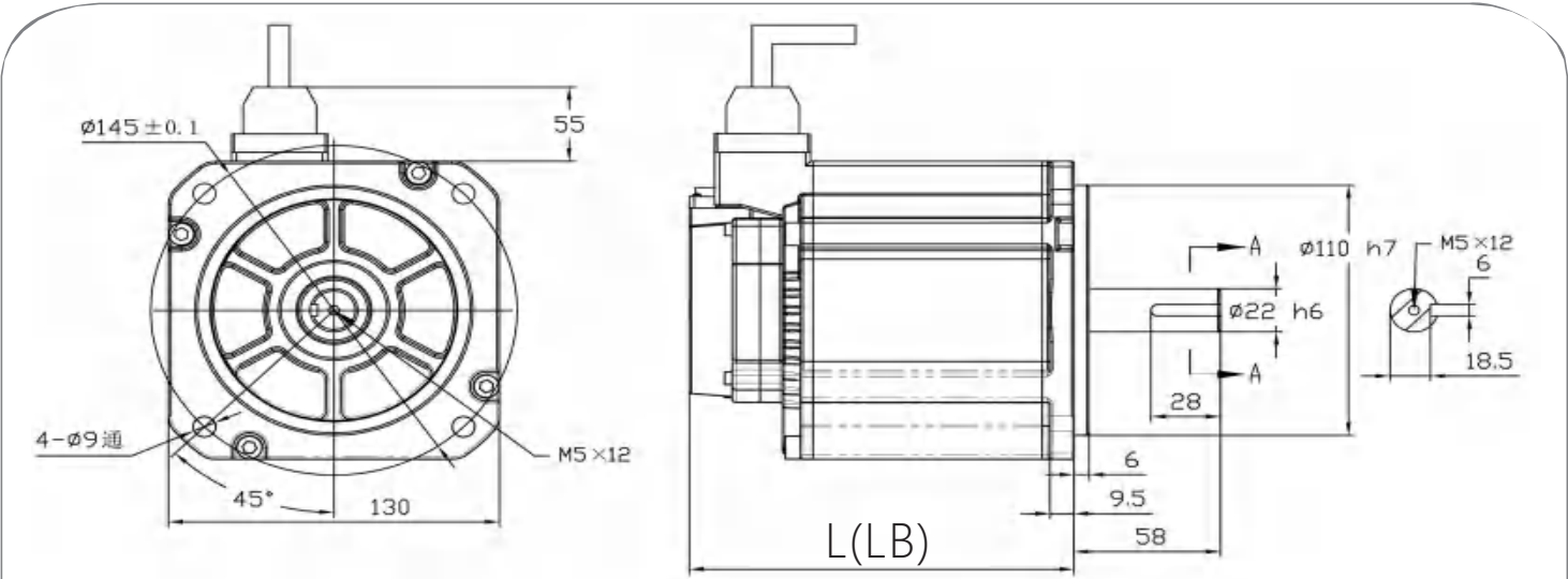
External Dimension
