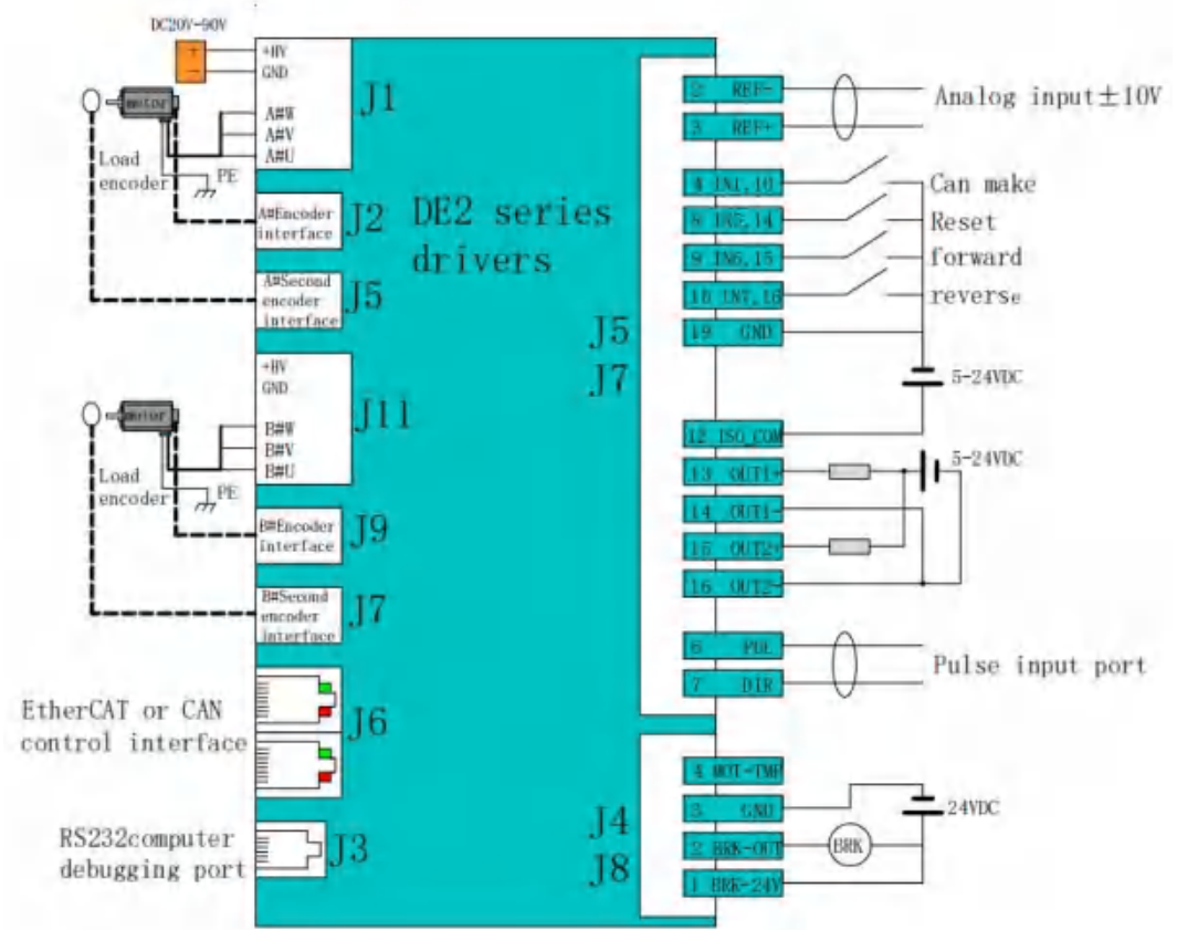
DE2 Typical wiring diagram
