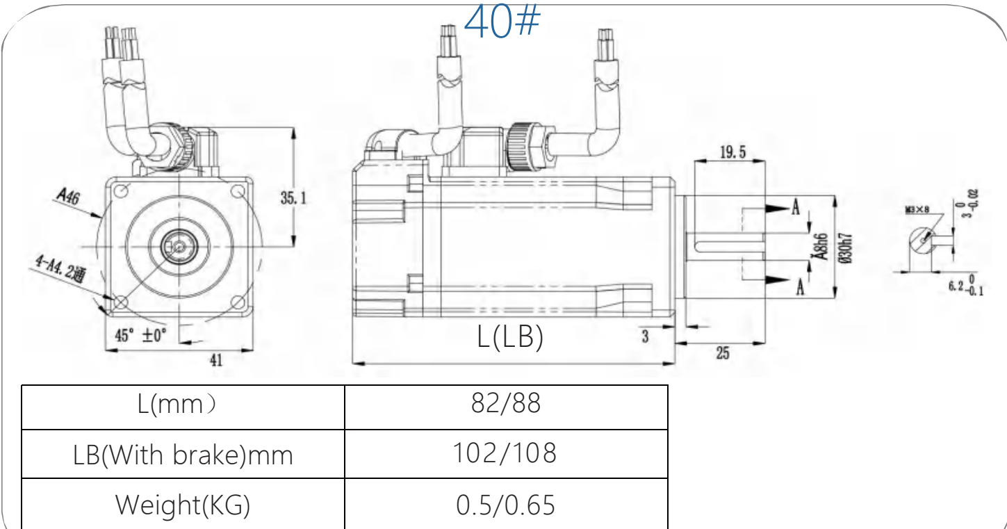
External Dimension
