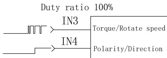
Figure 4.5.2 100% duty cycle + direction control
