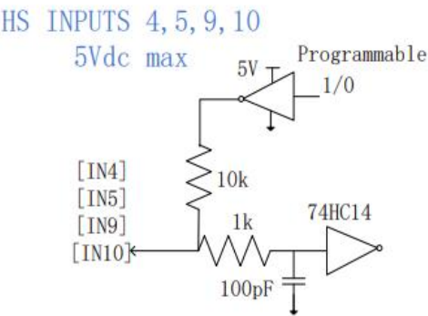
Figure 3.4.1 IN 1-IN 2 hardware input circuit Figure 3.4.2 High speed port hardware input circuit
