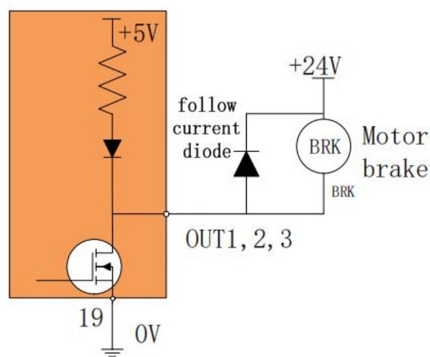
Figure 3.6.4 External circuit of motor lock brake
