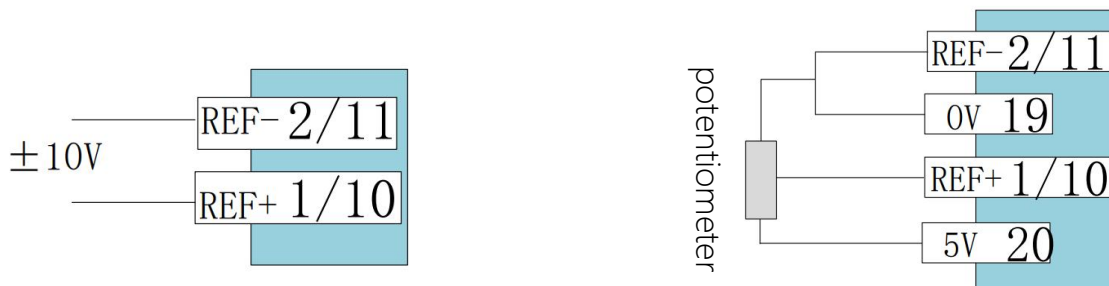
Figure 3.2.2 External power analog input cable
