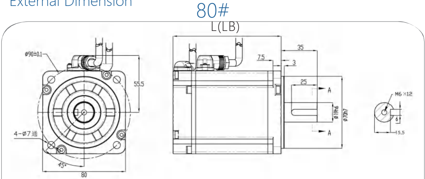
External Dimension
