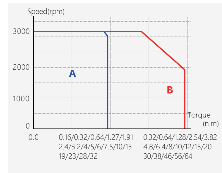
A:Continuous Duty Zone
