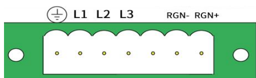
Figure 2.1.1 European gauge terminal socket
