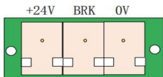
Figure 2.3 European gauge terminal socket
