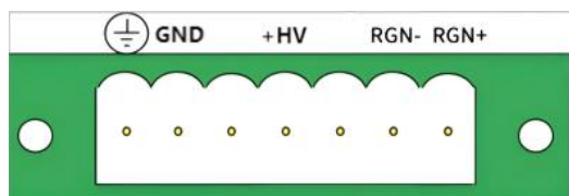
Figure 2.1.1 European Standard Terminal Sockets
